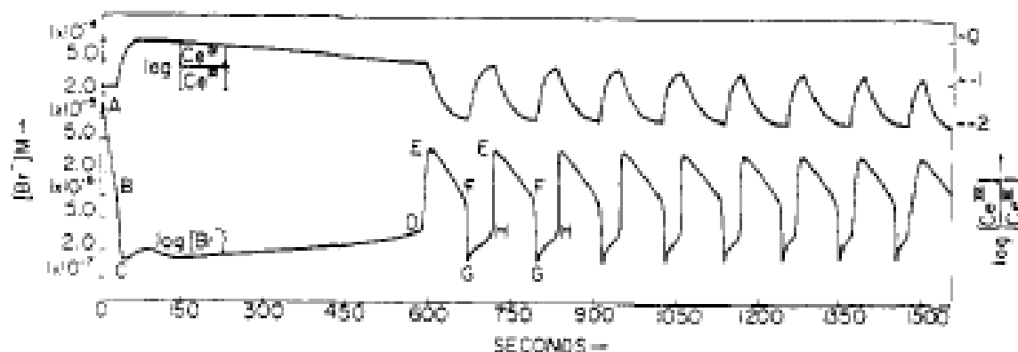
Figure 1. Potentiometric traces of \log [\text{Br}^-] and \log [\text{Ce(IV)}]/[\text{Ce(III)}] for a representative reaction exhibiting all six periods. Initial concentrations were [\text{CH}_3(\text{COOH})_2]_0 = 0.032 \text{ M} , [\text{KBrO}_3]_0 = 0.063 \text{ M} , [\text{KBr}]_0 = 1.5 \times 10^{-3} \text{ M} , [\text{Ce}(\text{NH}_4)_2(\text{NO}_3)_6]_0 = 0.001 \text{ M} , [\text{H}_2\text{SO}_4]_0 = 0.8 \text{ M} .
